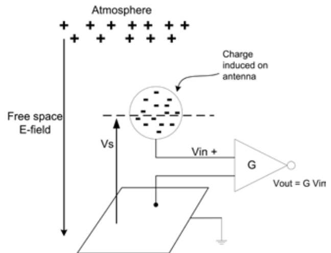
Figure 1. Measurement of the free-space electric potential by allowing a charge to flow onto a conducting test probe.
