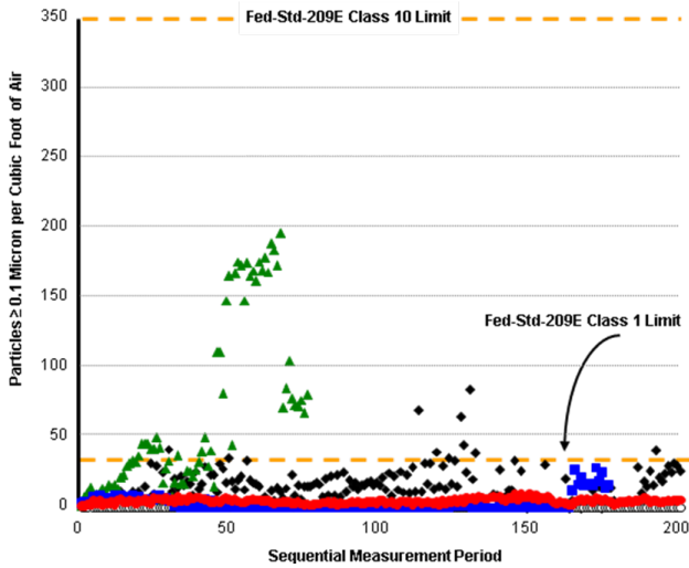
Figure 2. Particles \geq 0.1 Micron/Cubic Foot of Air vs. Sequential Measurement Period (Probe was 4 Inches Below the 5810i / 5802i Replacement Fans. Five fans were tested and shown in different colors)
