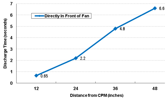
Figure 4. Model 5802i with NMB DC Axial Fan - Discharge Time
