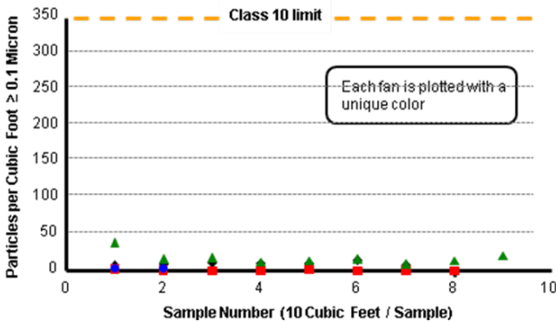
Figure 3. 5802i Particles/Cubic Foot of Air, \geq 0.1 Micron Measured 4" Below the Fan Stacks for 4 Fans (2 Units)
