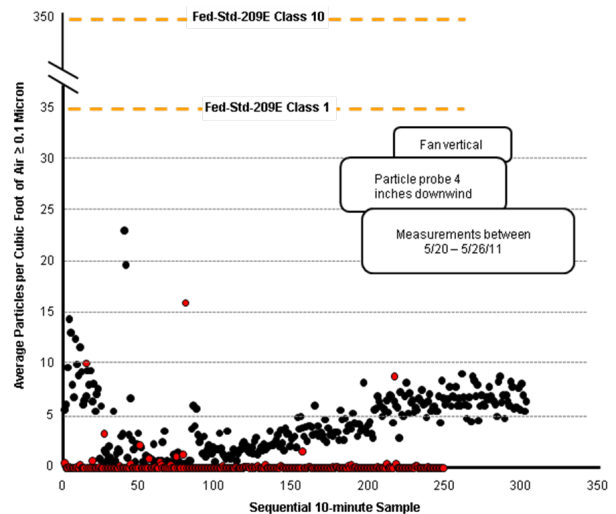
Figure 1. Particles \geq 0.1 Micron for NMB 5" Fans #5/6
