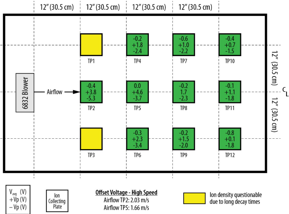
Figure 8. Offset Voltage Data – High Speed
