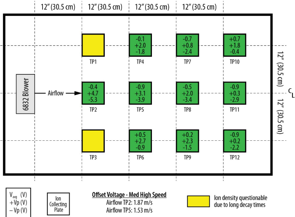
Figure 7. Offset Voltage Data – Medium-High Speed
