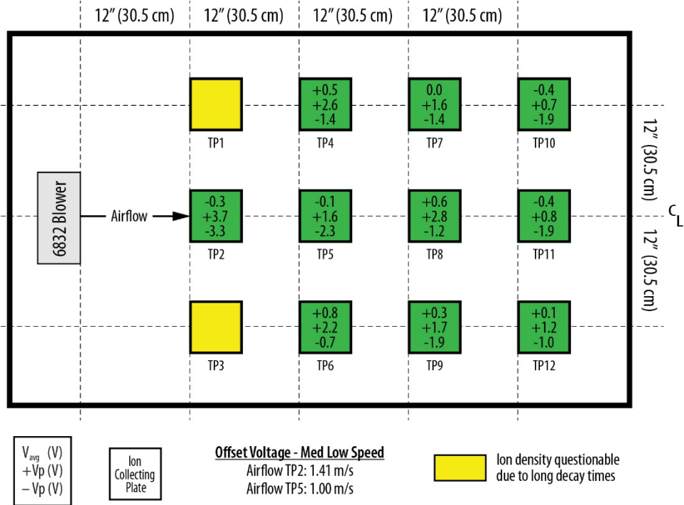
Figure 6. Offset Voltage Data – Medium-Low Speed
