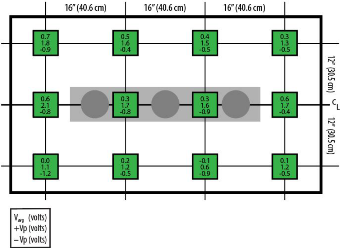
Figure 2. Offset Voltage Data
