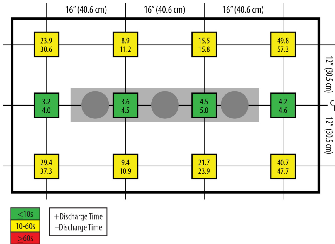
Figure 1. Discharge Time Data (±1000V to ±100V)
