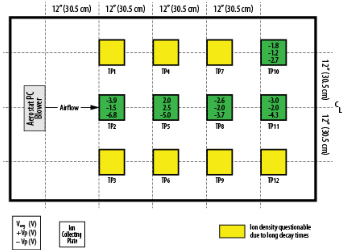
Figure 2. Offset Voltage Data – High Speed
