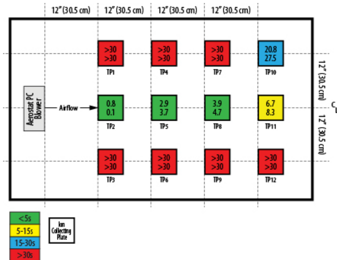
Figure 1. Discharge Time Data (±1000V to ±100V) – High Speed
