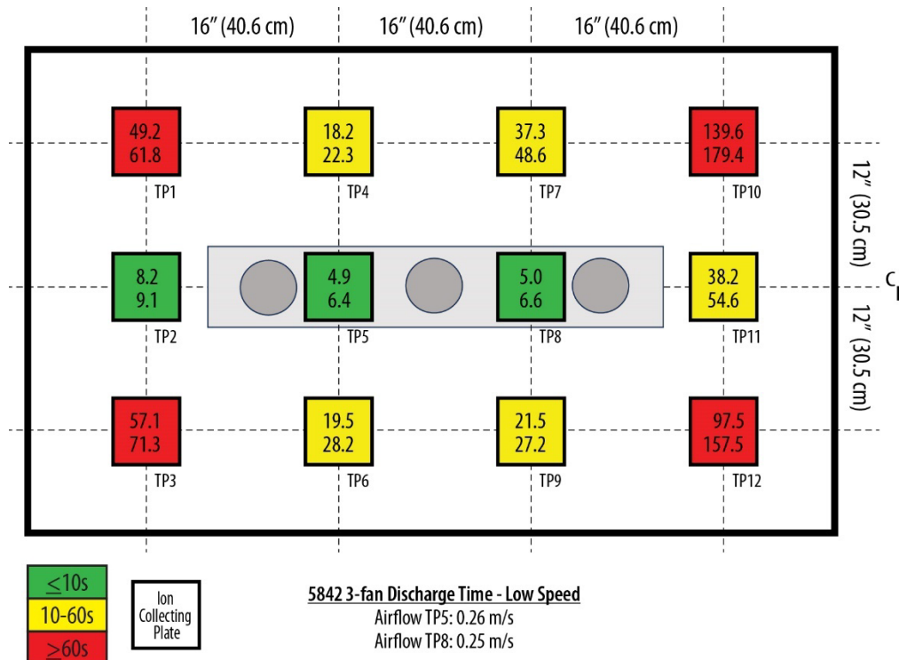
Figure 1. Discharge Time Data ( \pm 1000V to \pm 100V ) – Low Speed
